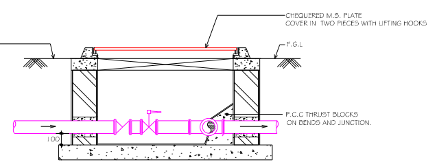
Section Valve Chamber
