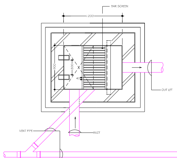
Plan Screen Chamber
