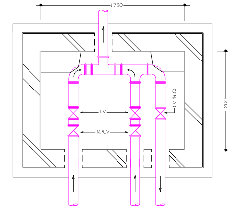
Plan Valve Chamber
