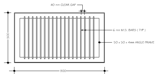
Details of Bar Screen
