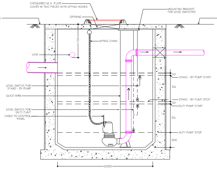
Section Sewage Collection Sump
