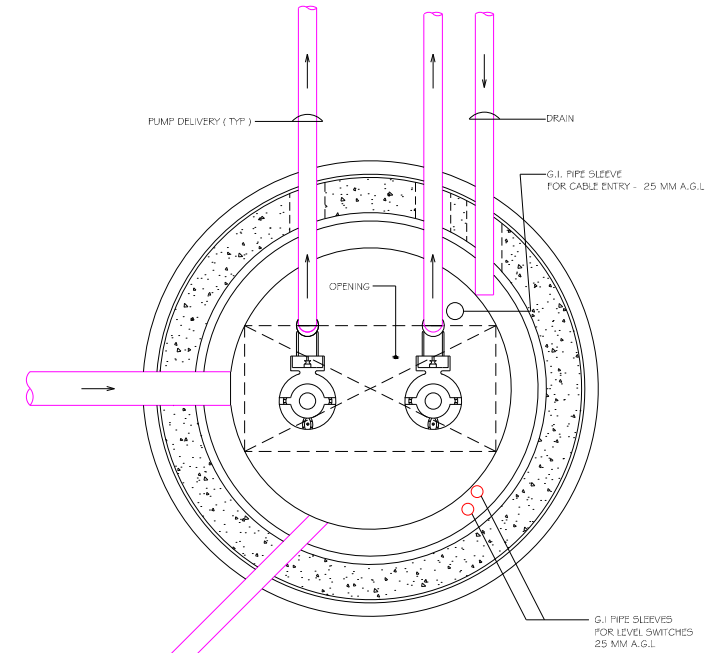
Plan Sewage Collection Sump
